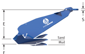
Dimensions in mm - Anchor weight in kg
